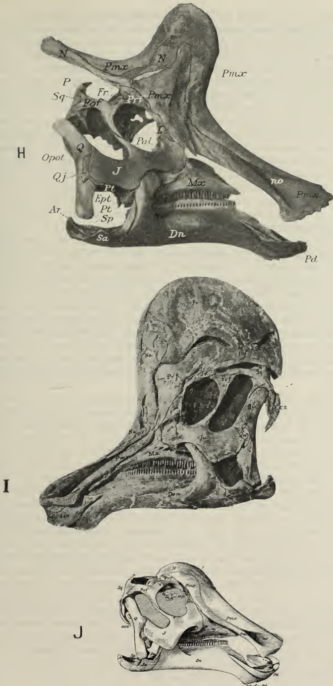
Figure 39. Skulls of Stephanosaurinae. H, Stephanosaurus , Lambe; I, Corythosaurus , Brown; J, Cheneosaurus , Lambe. \frac{1}{4} natural size.
